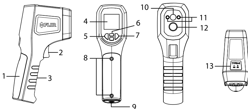
Figure 5.1 Meter Description
