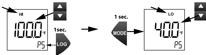
Figure 9.1 Setting the high and low alarm set points in the programming menu.
